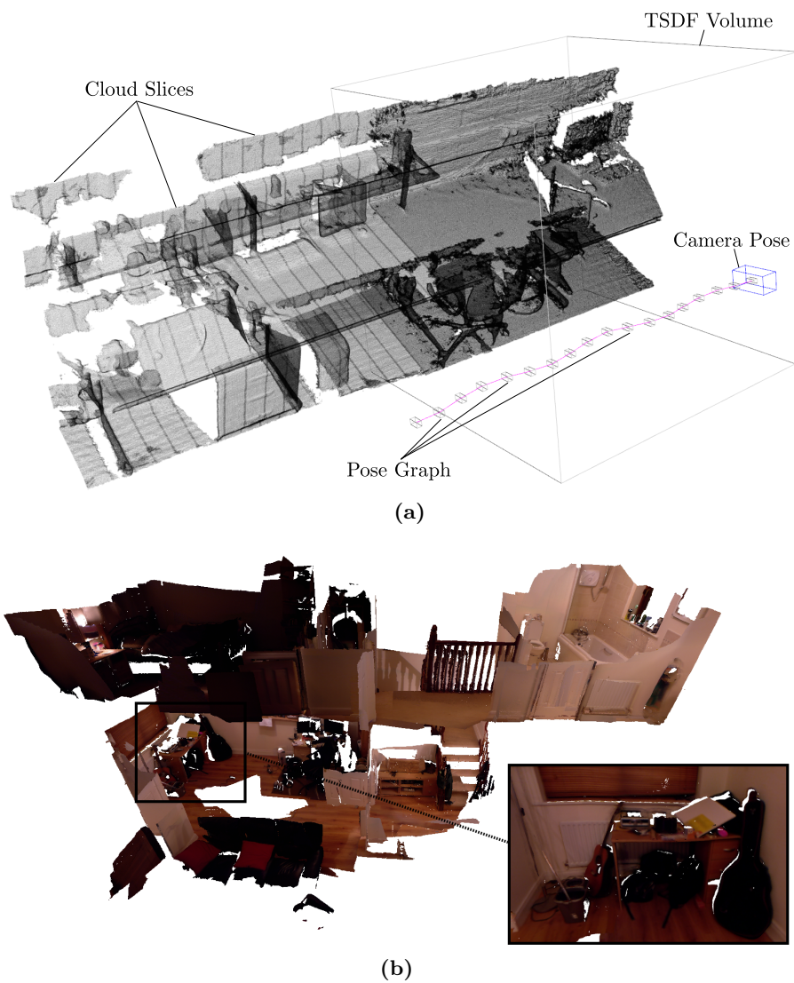
Figure 7.2: Real-time dense 3D mapping with Kintinuous [196]: (a) A dense volumetric representation (TSDF) is used locally and shifted along with the camera. The pose graph is drawn in pink with small cuboids as camera poses that have cloud slices associated with them. Loop closure on the pose graph is transferred to the point cloud via mesh deformation. (b) Sequence over two floors of an apartment with over six million vertices that was constructed including online loop closure. Small details such as bathroom fixtures and objects around the environment are clearly reconstructed.
