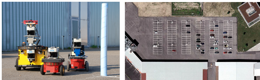
Figure 7.8: Three robots and a synthetic landmark used in the multi-robot mapping experiment from [35] (left), and an aerial view of the parking lot in which the experiment was performed (right).
