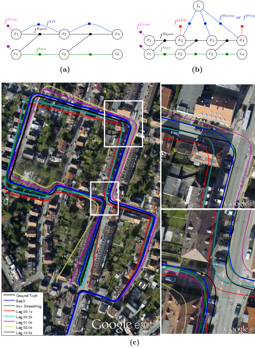
Figure 7.1: Aided inertial navigation [103]. (a) Factor graph for visual odometry integration with inertial bias estimation. (b) GPS integration (red factors) and/or stereo integration (blue). (c) Evaluation on KITTI sequence: Incremental smoothing performs almost as good as full batch optimization. Fixed-lag smoothing solutions are also shown for various lags.
