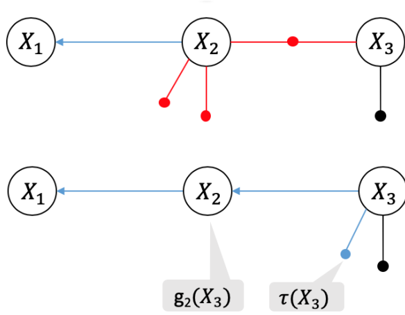
Figure 6: Max-product: eliminating X_2 .
