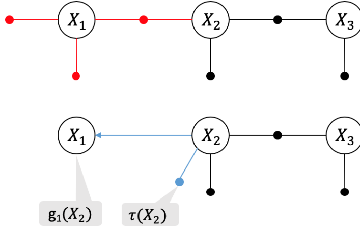
Figure 5: Max-product: eliminating X_1 .
