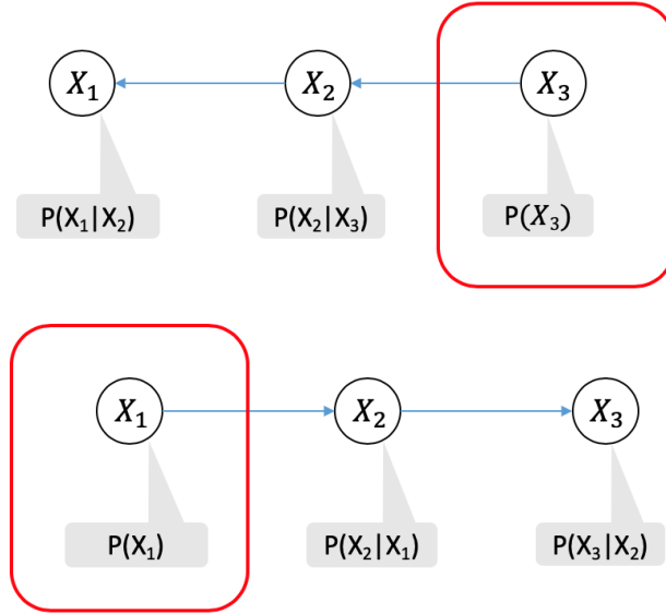
Figure 8: MAP estimation for X_3 and X_1 , respectively: we simply change the elimination order to make sure the variable(s) of interest are eliminated last.
